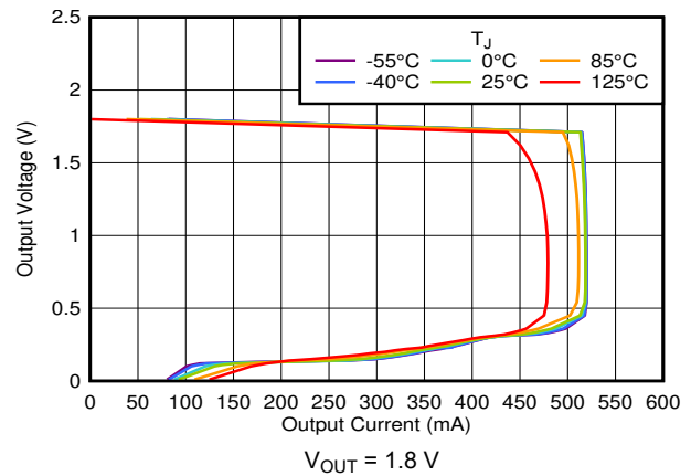
图 6-38. Foldback Current Limit vs I_{OUT} and Temperature
