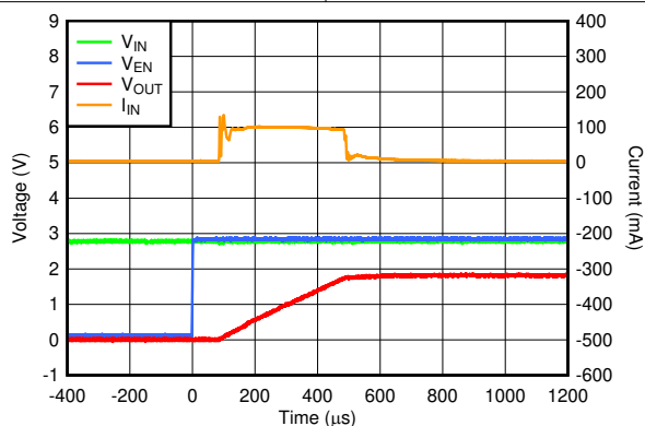
图 6-55. Startup With V_{EN} After V_{IN}
