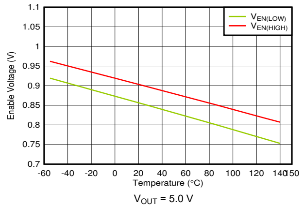
图 6-40. EN High and Low Threshold vs Temperature
