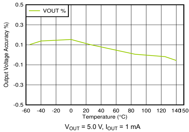
图 6-31. Output Accuracy vs Temperature
