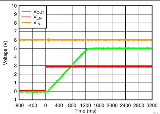
图 6-55. Startup With V_{EN} After V_{IN}
