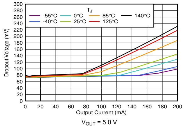
图 6-34. Dropout vs I_{OUT} and Temperature
