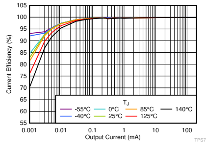
图 8-5. Current Efficiency vs I_{OUT} and Temperature
