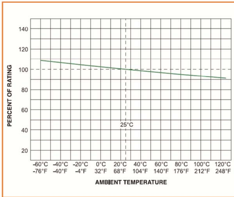
Temperature Derating Curve
