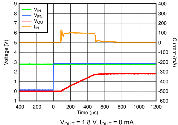
图 6-56. Startup Inrush Current With C_{OUT} = 22\text{ }\mu\text{F}
