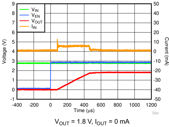
图 6-55. Startup Inrush Current With C_{OUT} = 1\text{ }\mu\text{F}
