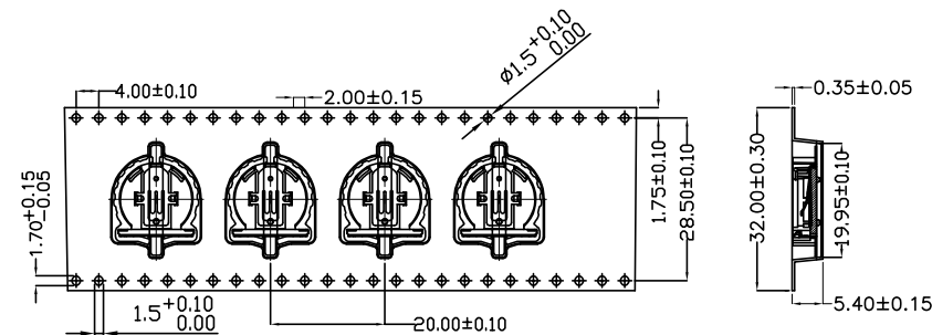
Detail A
