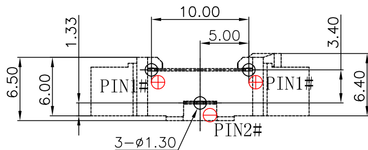
PCB Layout Diagram Bottom View
