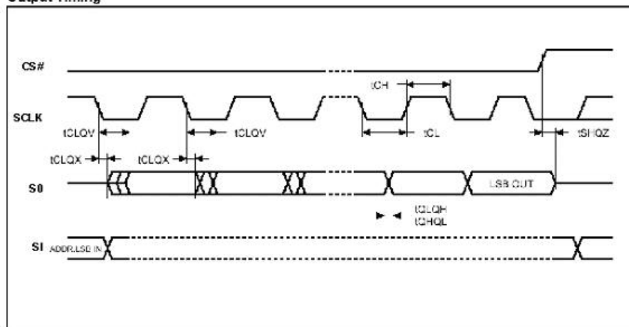
Output Timing
