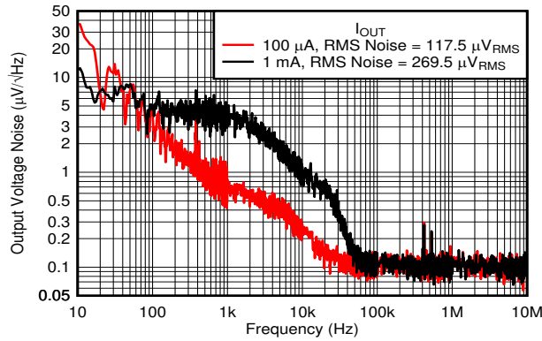
图 6-49. Output Noise vs Frequency and I_{OUT}
