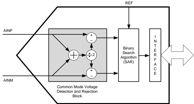
Figure 40. Conceptual Diagram: True Differential Input Structure
