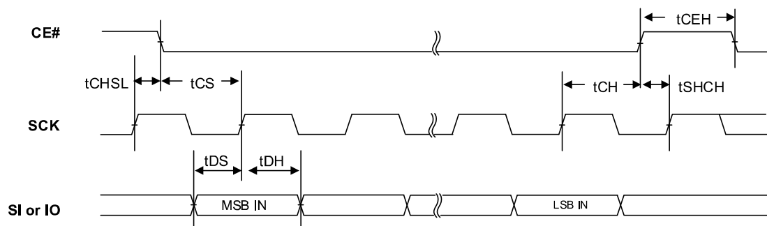
Figure 9.2 SERIAL INPUT TIMING (STR Mode)
