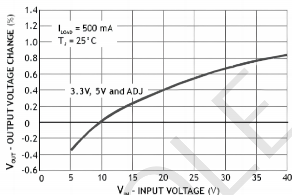
LINE REGULATION
