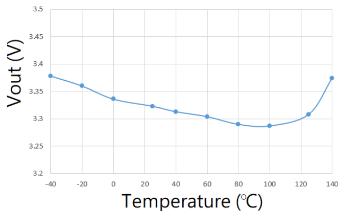
Fig 9. V_{OUT} vs 温度 ( I_{OUT} = 1mA )
