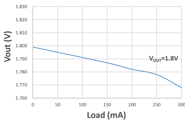
Fig 12. V_{OUT} vs 负载
