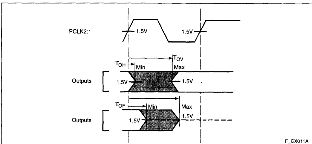
Figure 10. Output Delay and Float Waveform
