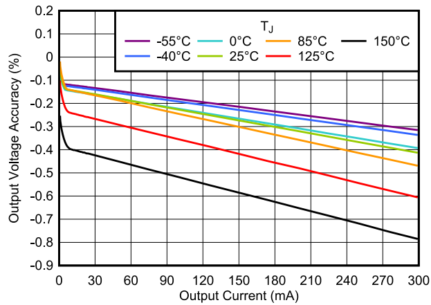
V_{OUT} = 5.5 \text{ V} , V_{EN} = 1 \text{ V} , DBV package Figure 5-19. Output Voltage Accuracy vs I_{OUT}
