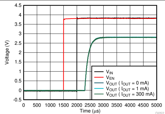
Figure 5-76. Start-Up
