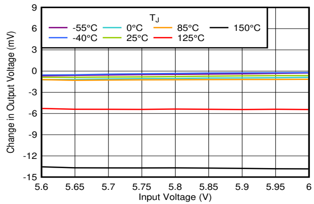
Figure 5-2. Line Regulation vs V_{IN}
