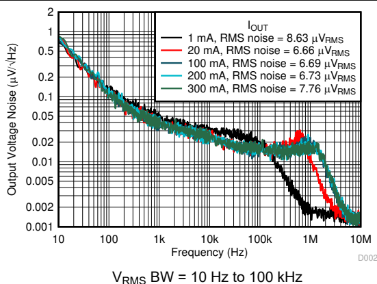
Figure 5-65. Noise vs Frequency and I_{OUT}
