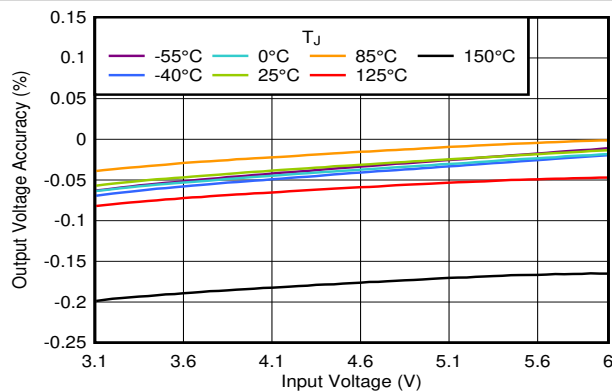
V_{EN} = 1 \text{ V} , I_{OUT} = 1 \text{ mA} , DQN, YCJ, and YCK packages Figure 5-21. Output Voltage Accuracy vs V_{IN}
