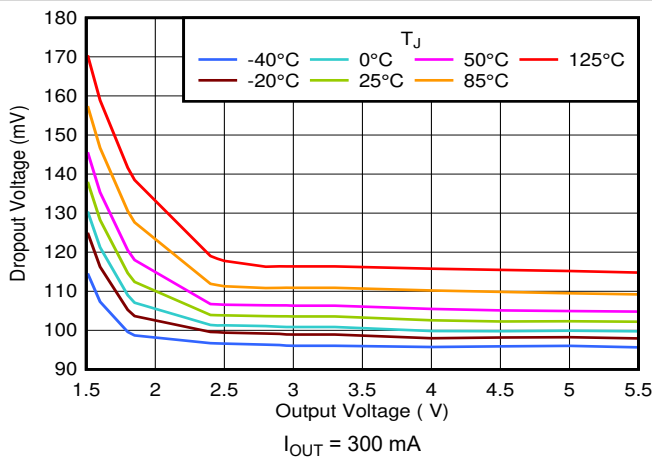
Figure 5-33. Dropout Voltage vs V_{OUT}
