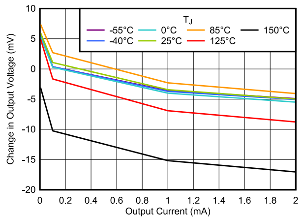
V_{OUT} = 5.5 \text{ V} , V_{EN} = 1 \text{ V} , DBV package Figure 5-12. Load Regulation vs I_{OUT}
