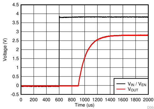
Figure 7-5. Start-Up
