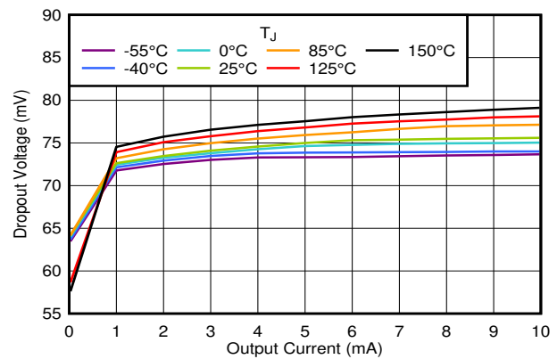
Figure 5-26. Dropout Voltage vs I_{OUT}
