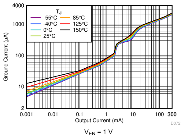
Figure 5-39. I_{GND} vs I_{OUT}
