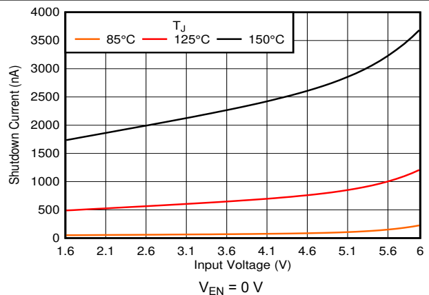
Figure 5-42. Shutdown Current vs V_{IN}
