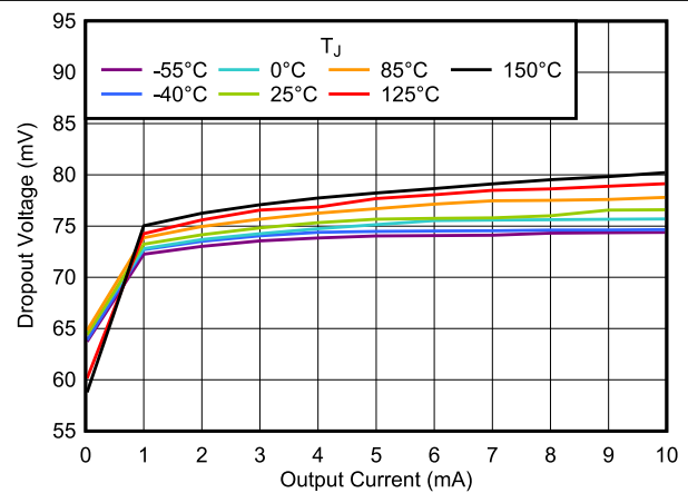
Figure 5-28. Dropout Voltage vs I_{OUT}
