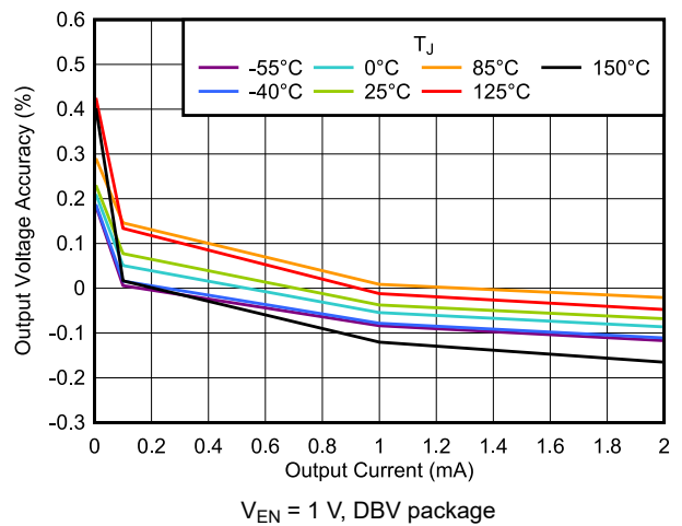
Figure 5-16. Output Voltage Accuracy vs I_{OUT}
