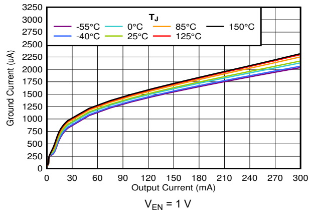
Figure 5-38. I_{GND} vs I_{OUT}
