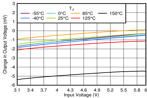
Figure 5-1. Line Regulation vs V_{IN}
