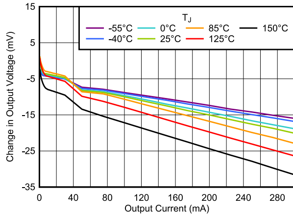
V_{IN} = 2.8 \text{ V} , V_{EN} = 1 \text{ V} , DBV package Figure 5-7. Load Regulation vs I_{OUT}
