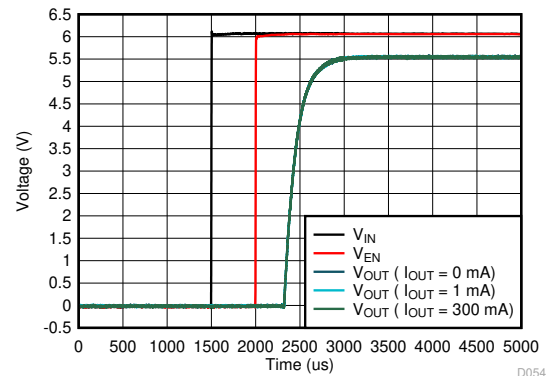
Figure 5-80. Start-Up
