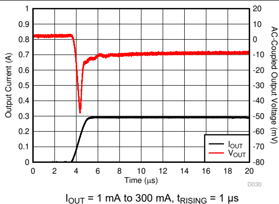
Figure 5-51. Load Transient
