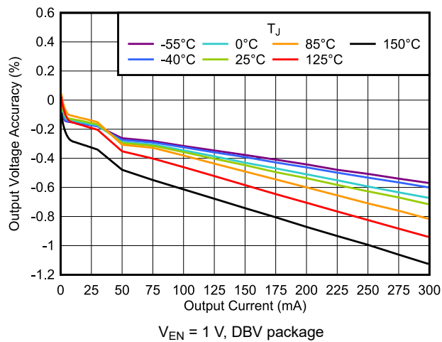
Figure 5-15. Output Voltage Accuracy vs I_{OUT}
