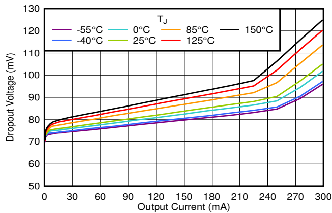
Figure 5-25. Dropout Voltage vs I_{OUT}
