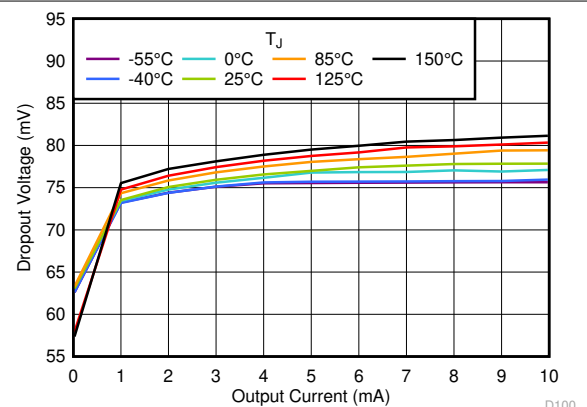
Figure 5-28. Dropout Voltage vs I_{OUT}
