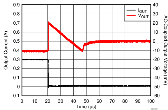
Figure 5-52. Load Transient
