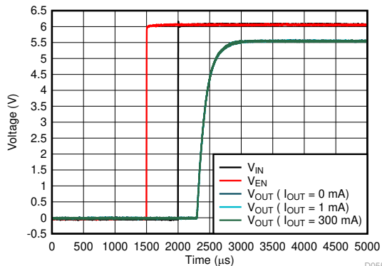
Figure 5-79. Start-Up
