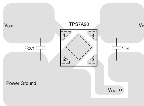
Figure 7-8. DQN Package (X2SON) Typical Layout
