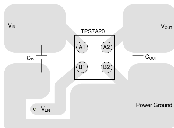
Figure 7-9. YCJ and YCK Package (DSBGA) Typical Layout
