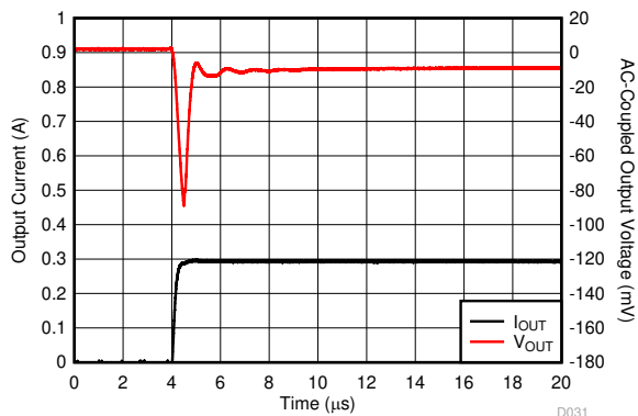
Figure 5-51. Load Transient
