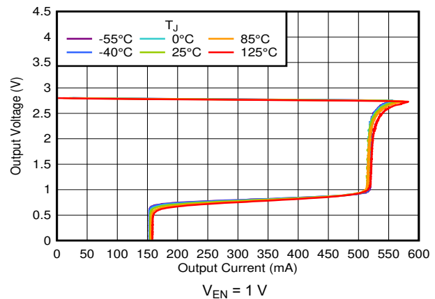
Figure 5-44. Current Limit
