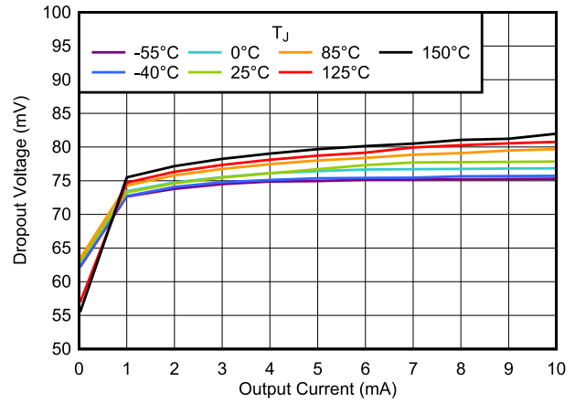
Figure 5-32. Dropout Voltage vs I_{OUT}
