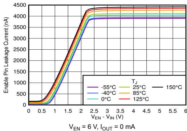
Figure 5-43. Enable Pin Leakage Current vs V_{EN} - V_{IN}
