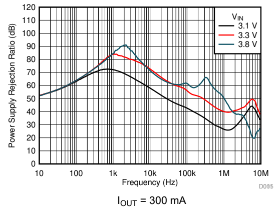
Figure 5-62. PSRR vs Frequency and V_{IN}
