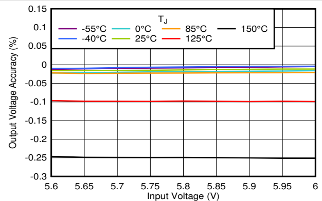
V_{OUT} = 5.5 \text{ V} , V_{EN} = 1 \text{ V} , DQN, YCJ, and YCK packages Figure 5-22. Output Voltage Accuracy vs V_{IN}
