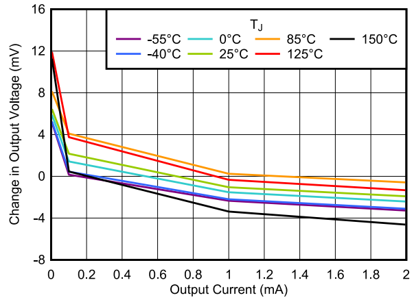
V_{IN} = 2.8 \text{ V} , V_{EN} = 1 \text{ V} , DBV package Figure 5-8. Load Regulation vs I_{OUT}
