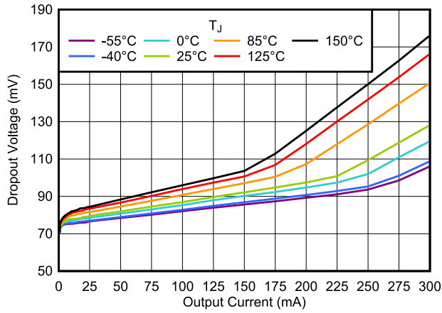
Figure 5-31. Dropout Voltage vs I_{OUT}
