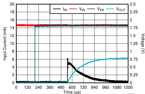
Figure 5-81. Start-Up
