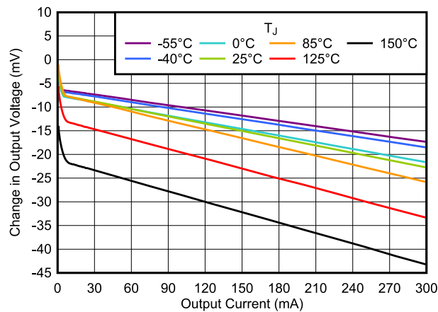
V_{OUT} = 5.5 \text{ V} , V_{EN} = 1 \text{ V} , DBV package Figure 5-11. Load Regulation vs I_{OUT}
