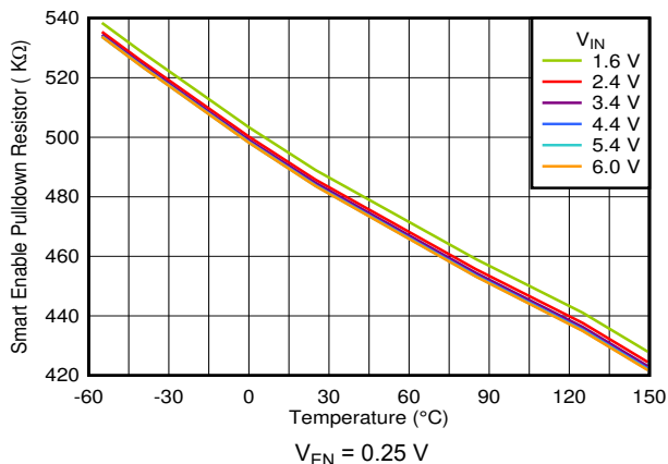
Figure 5-50. Smart Enable Pulldown Resistor vs Temperature and V_{IN}
