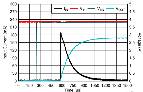
Figure 5-82. Start-Up
