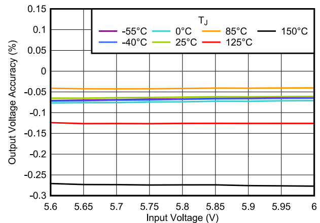
V_{OUT} = 5.5 \text{ V} , V_{EN} = 1 \text{ V} , DBV package Figure 5-24. Output Voltage Accuracy vs V_{IN}
