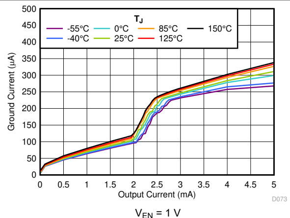
Figure 5-40. I_{GND} vs I_{OUT}
