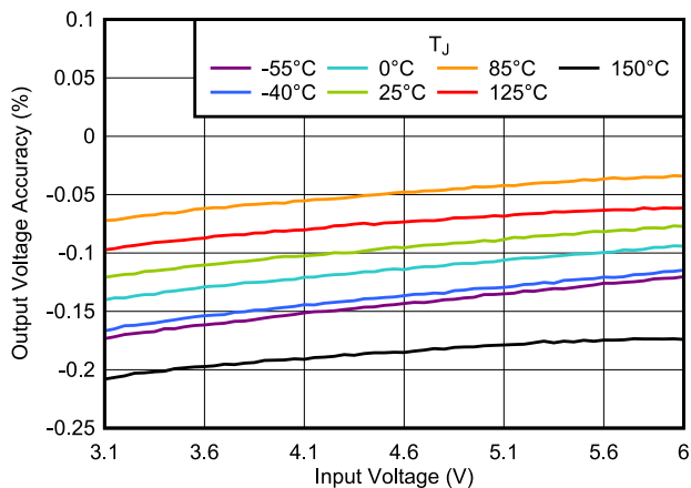
V_{EN} = 1 \text{ V} , I_{OUT} = 1 \text{ mA} , DBV package Figure 5-23. Output Voltage Accuracy vs V_{IN}
