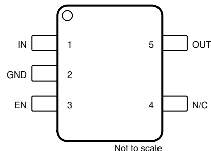
Figure 4-4. DBV Package, 5-Pin SOT-23 (Top View)
