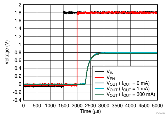
Figure 5-74. Start-Up
