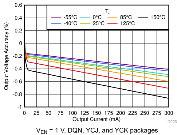
Figure 5-13. Output Voltage Accuracy vs I_{OUT}
