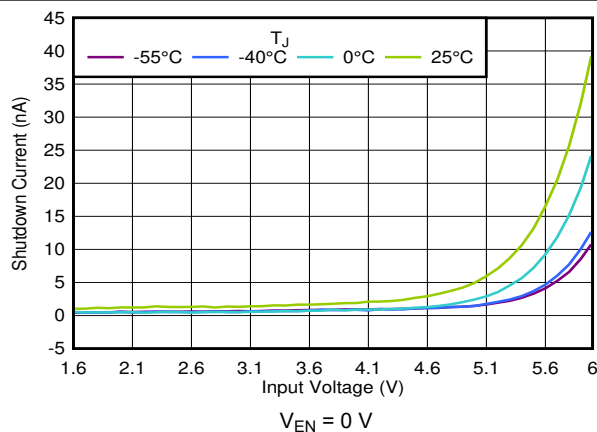
Figure 5-41. Shutdown Current vs V_{IN}
