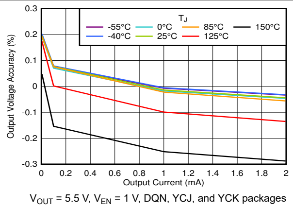
Figure 5-18. Output Voltage Accuracy vs I_{OUT}
