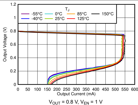
Figure 5-45. Current Limit
