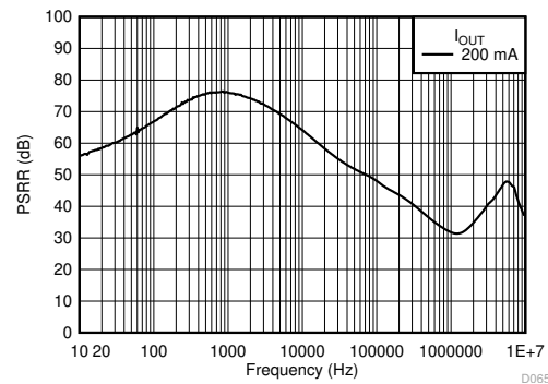
Figure 7-6. PSRR
