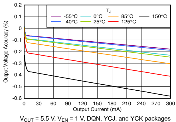
Figure 5-17. Output Voltage Accuracy vs I_{OUT}
