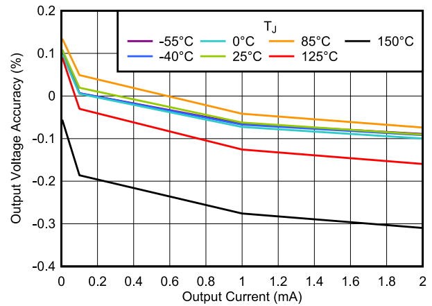
V_{OUT} = 5.5 \text{ V} , V_{EN} = 1 \text{ V} , DBV package Figure 5-20. Output Voltage Accuracy vs I_{OUT}
