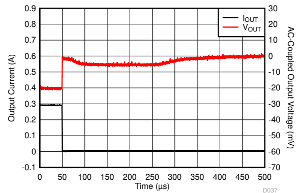
Figure 5-56. Load Transient
