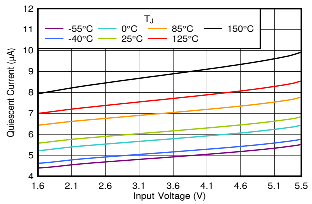
Figure 5-36. I_{GND} vs V_{IN} in the Dropout Region
