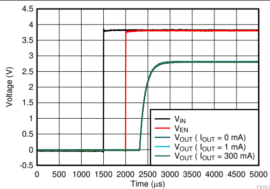
Figure 5-75. Start-Up
