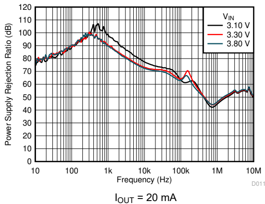
Figure 5-61. PSRR vs V_{IN} vs Frequency and V_{IN}
