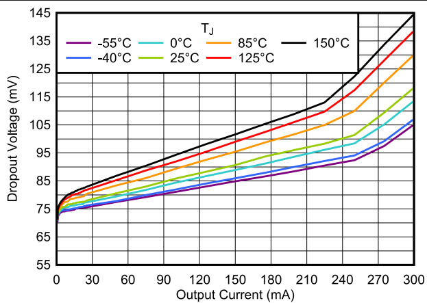
Figure 5-25. Dropout Voltage vs I_{OUT}
