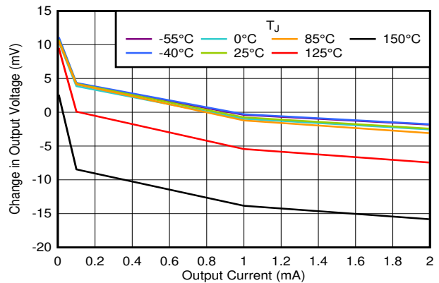
V_{IN} = 2.8 \text{ V} , V_{EN} = 1 \text{ V} , DBV package Figure 5-8. Load Regulation vs I_{OUT}
