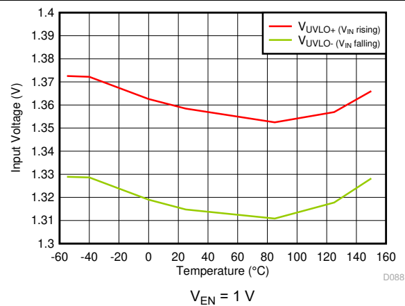
Figure 5-46. UVLO Threshold vs Temperature
