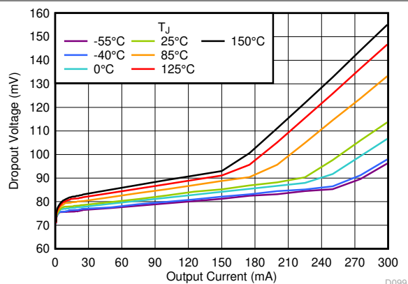
Figure 5-27. Dropout Voltage vs I_{OUT}
