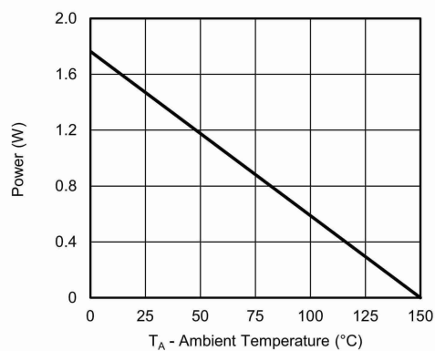
Power, Junction-to-Ambient
