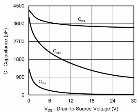
Capacitance
