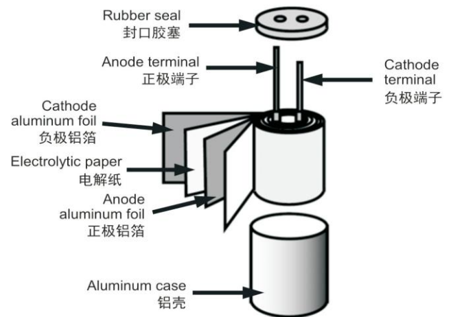
(Basic construction 基本结构)
