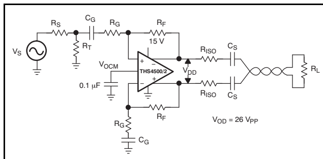
Figure 105. Fully Differential Line Driver With High Output Swing
