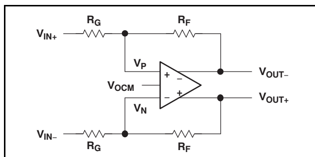
Figure 101. Diagram For Input Common-Mode Range Equations
