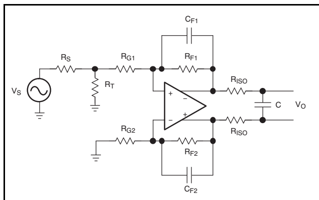
Figure 106. A Two-Pole, Low-Pass Filter Design Using a Fully Differential Amplifier With Poles Located at: P1 = (2\pi R_F C_F)^{-1} in Hz and P2 = (4\pi R_{ISO} C)^{-1} in Hz
