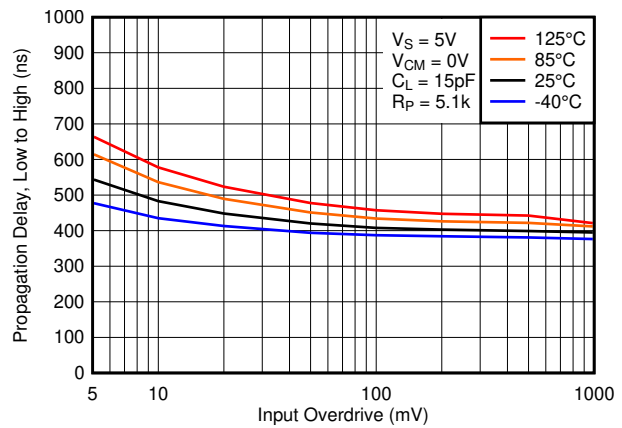
图 6-26. Low to High Propagation Delay vs. Input Overdrive Voltage, 5V
