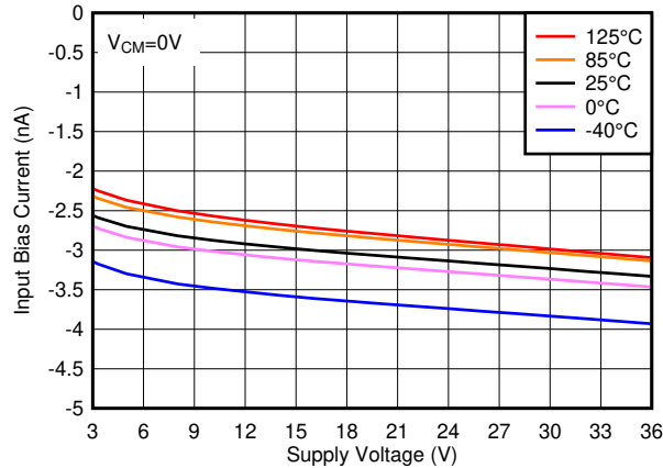
图 6-15. Input Bias Current vs. Supply Voltage
