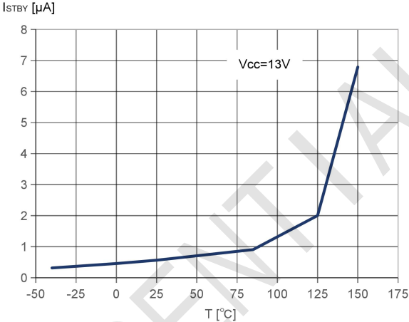
Standby current
