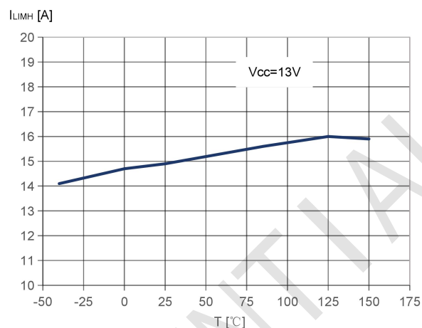
I_{LMH} vs. T_A
