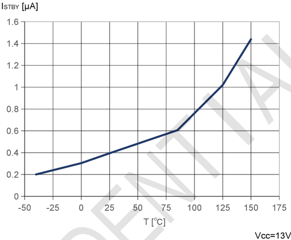
Standby current
