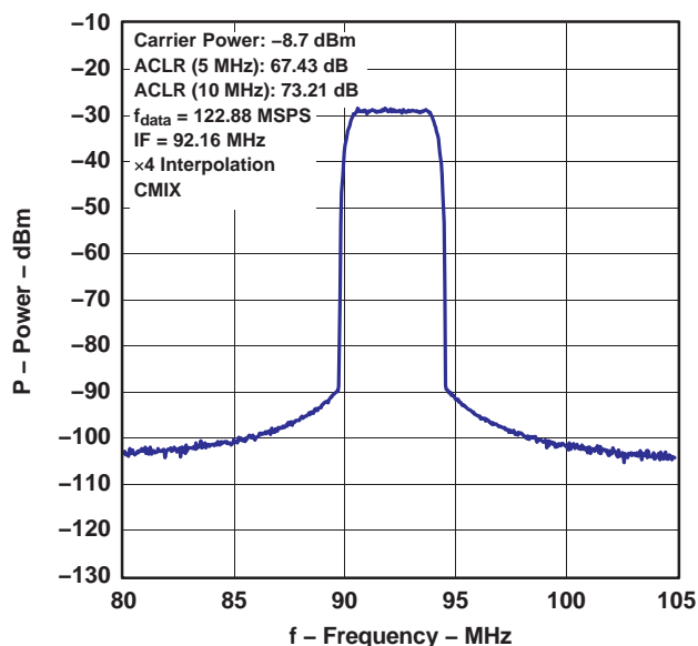
Figure 17. WCDMA TM1 : Single Carrier, PLL On, DVDD = 1.8 V
