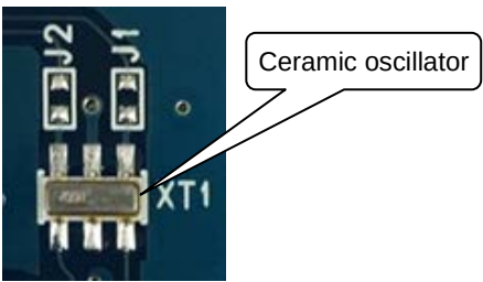
Figure 4 Ceramic resonator
