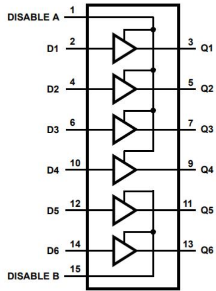
Figure 2.2 Functional Diagram
