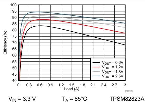
图 9-142. Efficiency
