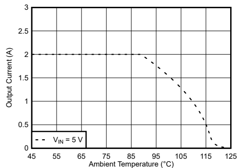
图 9-98. Safe Operating Area
