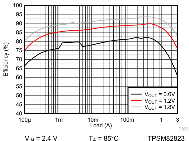
图 9-117. Efficiency
