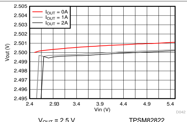
图 9-74. Line Regulation
