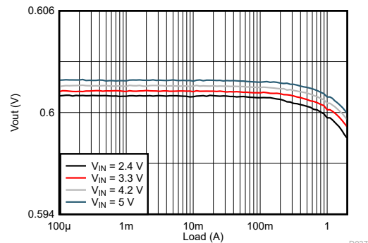
图 9-99. Load Regulation
