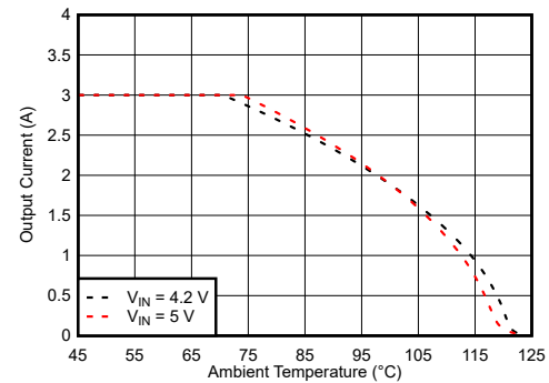
图 9-146. Safe Operating Area
