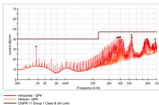
图 9-136. TPSM82823 Radiated Emissions
