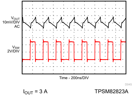
图 9-155. Output Ripple in PWM Mode
