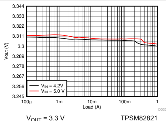
图 9-20. Load Regulation
