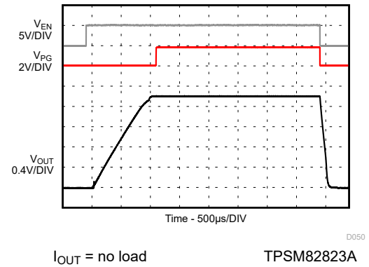
图 9-158. Start-up / Shutdown without Load
