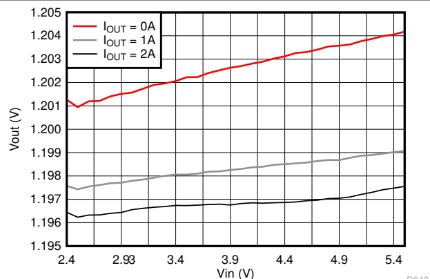
图 9-72. Line Regulation
