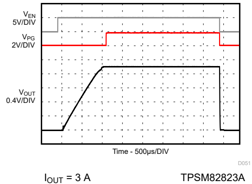
图 9-159. Start-up / Shutdown with Resistive Load
