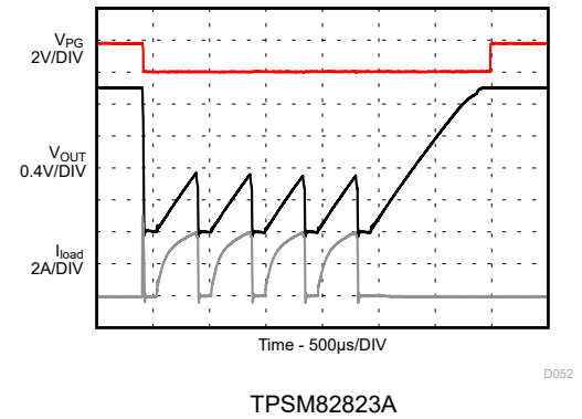
图 9-160. Short Circuit, HICCUP Protection Entry / Exit
