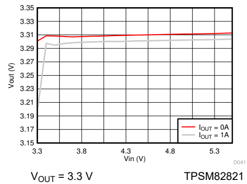
图 9-24. Line Regulation
