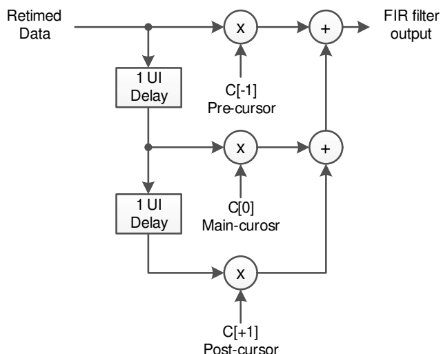
图 6-3. FIR filter functional model
