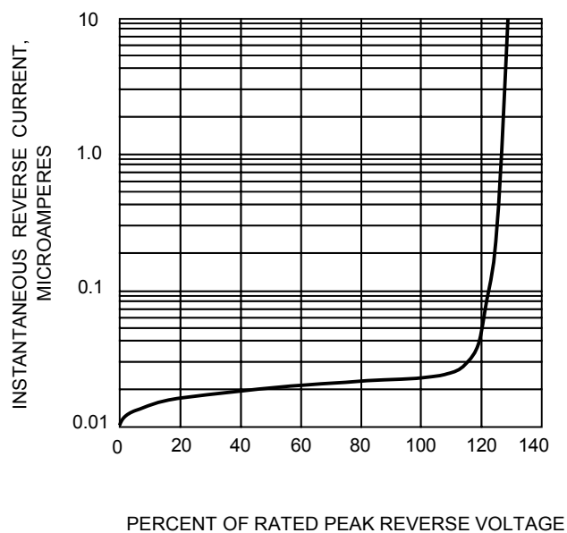
FIG.4-TYPICAL REVERSE CHARACTERISTICS
