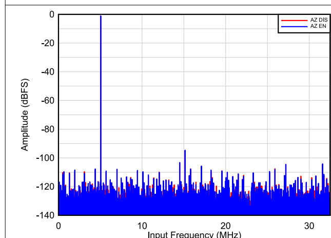
图 8-12. F_S = 65 MSPS, F_{IN} = 5 MHz
