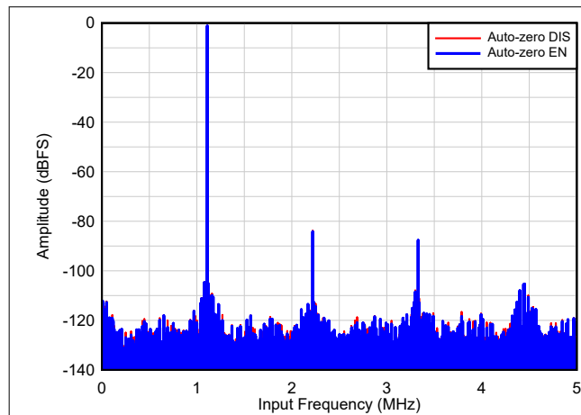
图 8-8. F_S = 10 MSPS, F_{IN} = 1.1 MHz
