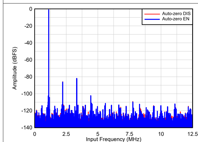
图 8-10. F_S = 25 MSPS, F_{IN} = 1.1 MHz
