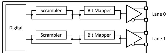
图 8-46. Output scrambling per lane
