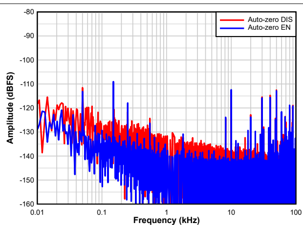
图 8-9. F_S = 10 MSPS, F_{IN} = 1.1 MHz
