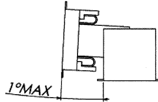
図4/ Fig.4(垂直接続タイプに適用/ Apply to vertical connection)
