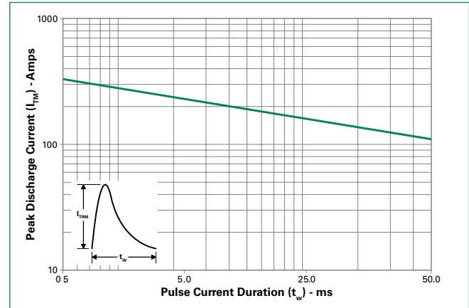
Figure 8: Peak Capacitor Discharge Current
