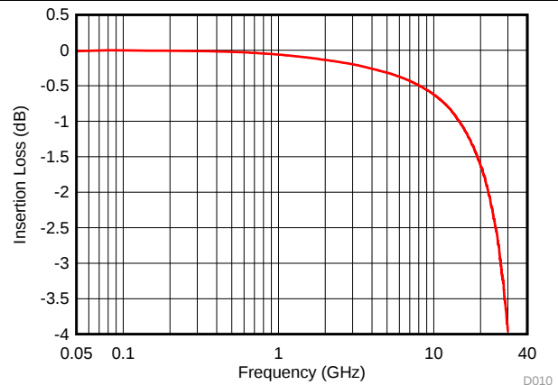
Figure 10. Insertion Loss
