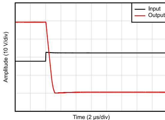
图 5-30. Negative Overload Recovery
