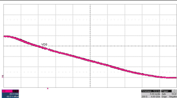
图 8-10. Slew Rate Adjust SRF = 100 \Omega
