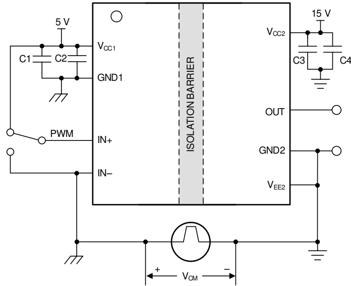
图 7-5. CMTI Test Circuit for UVLO2 with Respect to GND2 (UCC53x0E)
