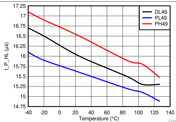
图 41. Propagation Detect Time Delay for V_{DD} Falling Below V_{IT} . (High-to-Low) over Temperature
