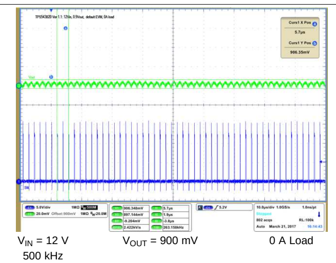
图 8. Output Voltage Ripple at Steady State
