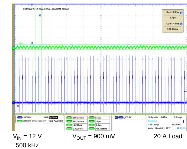
图 9. Output Voltage Ripple at Steady State
