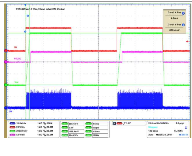
图 12. Output Voltage Start-Up and Shutdown
