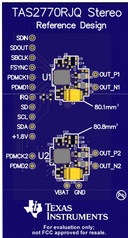
图 11-2. Stereo EVM Layout Reference Design - 01
