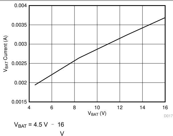
图 6-17. V BAT Idle Current vs V BAT
