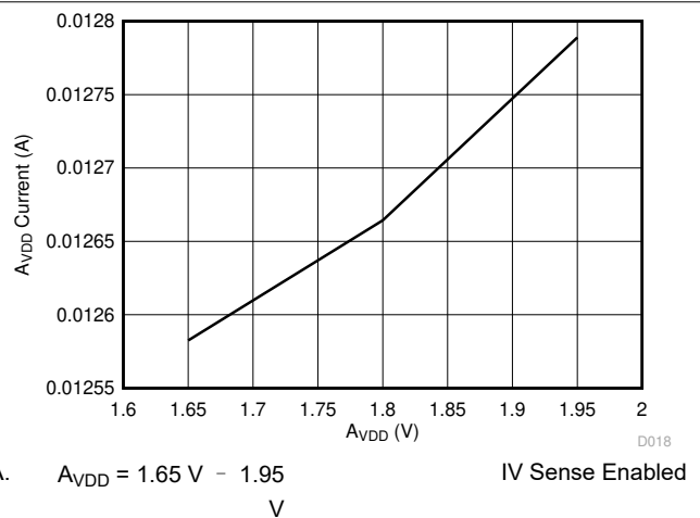
图 6-18. A VDD Idle Current vs A VDD
