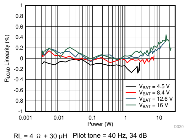
图 6-29. V_{\text{I\_SENSE}} Gain Linearity vs Output Power
