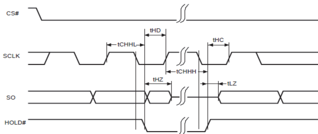
Figure 4.3 Hold Timing
