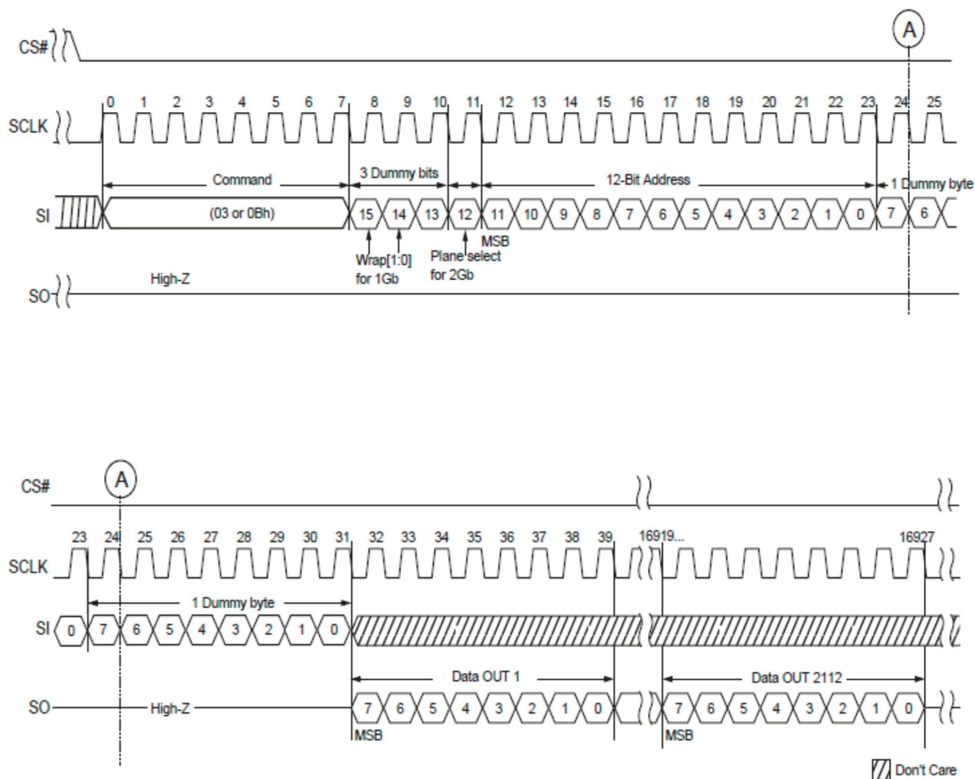
Figure 3.6 Random Data Read (03h or 0Bh)
