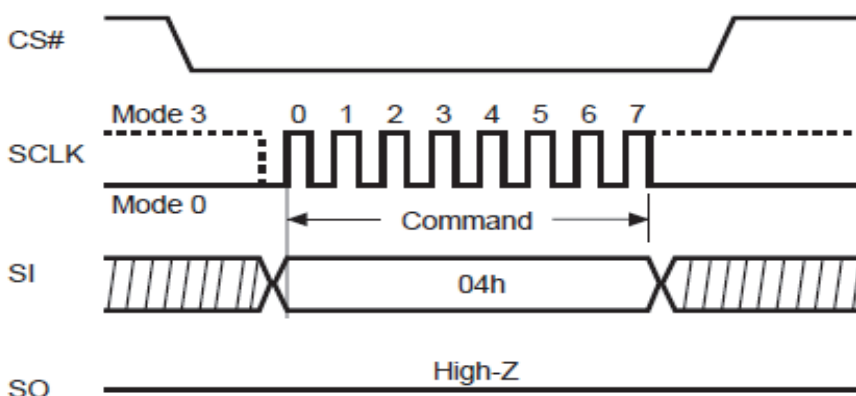
Figure 3.2 Write Disable
