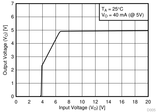
图 8-4. Output Voltage vs Input Voltage for Legacy Chip
