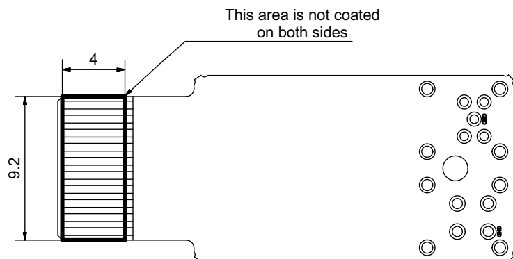
Figure 7 PCB Contact Pad Area
