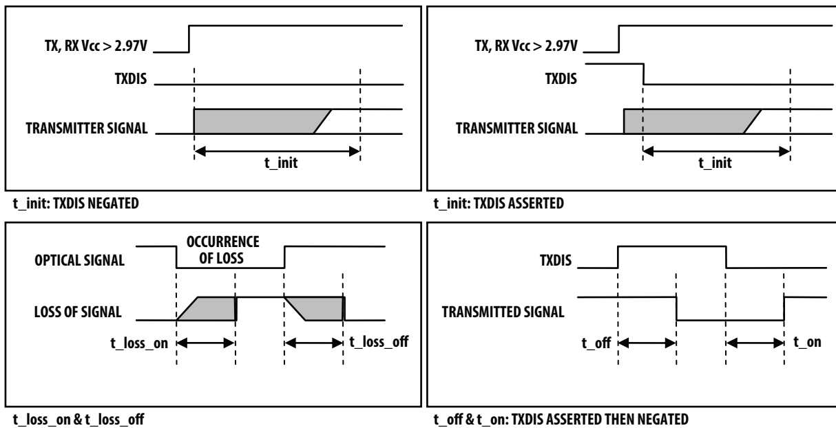
Figure 9 Timing Diagram
