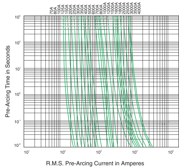
Average Time-Current Curve
