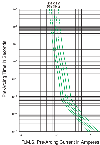
Average Time-Current Curve
