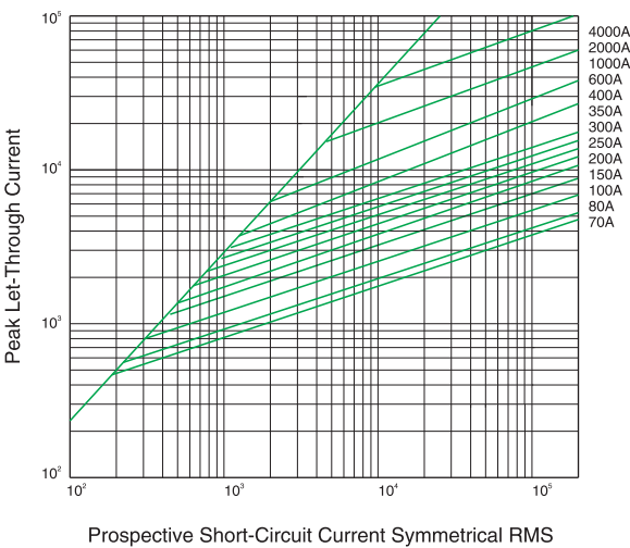
Peak Let -Thru Curve
