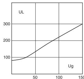
Arc Voltage
