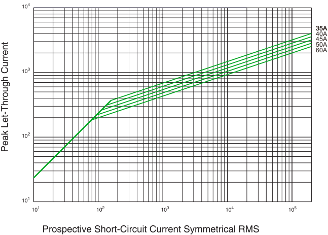
Peak Let -Thru Curve
