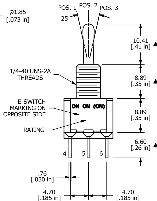
P.C. MOUNTING
