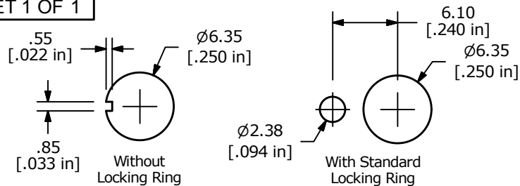
PANEL MOUNTING
