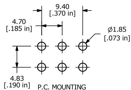
P.C. MOUNTING
