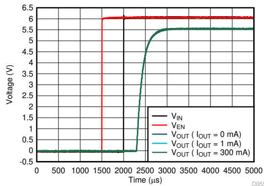
图 5-79. Start-Up
