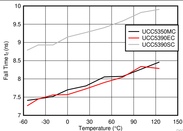
图 6-30. Fall Time vs Temperature
