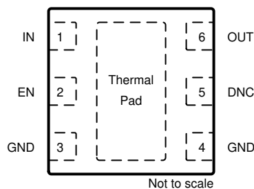
图 5-2. DRV Package, 6-Pin WSON (Top View)
