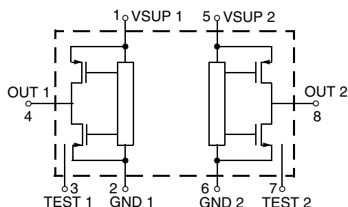
Fig. 4–2: Pin configuration
