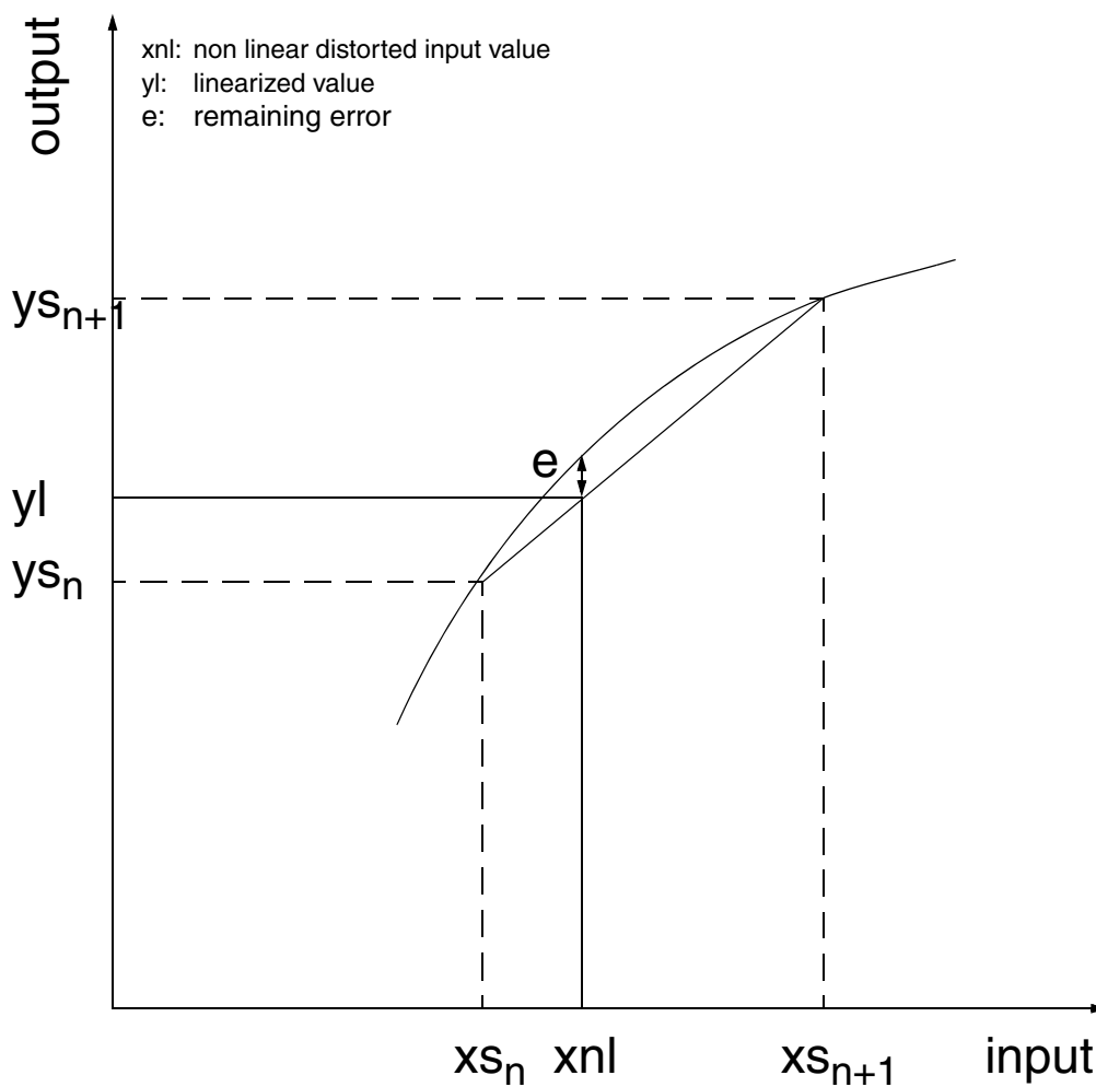
Fig. 3–6: Linearization - detail
