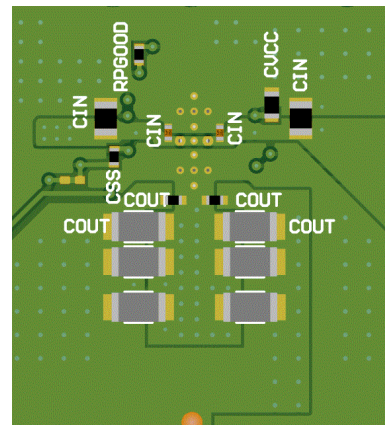
图 10-2. Recommended Layout Bottom Side
