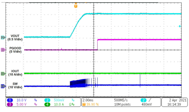
图 8-31. Startup Through V_{IN} (Enable Floating)
