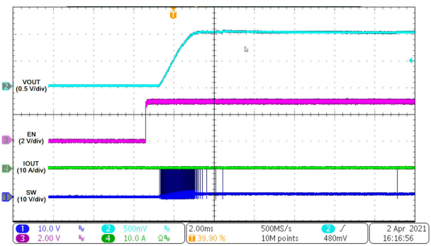
图 8-33. Startup Through Enable
