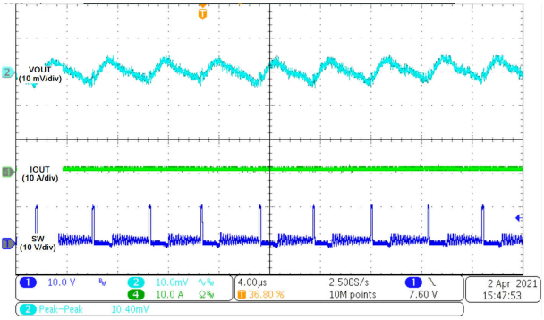
图 8-29. Output Voltage Ripple, V_{RIPPLE} = 10.4\text{ mV}
