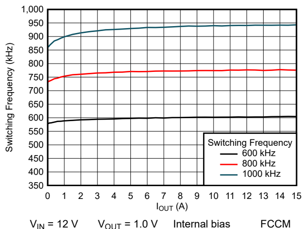
图 8-20. Switching Frequency
