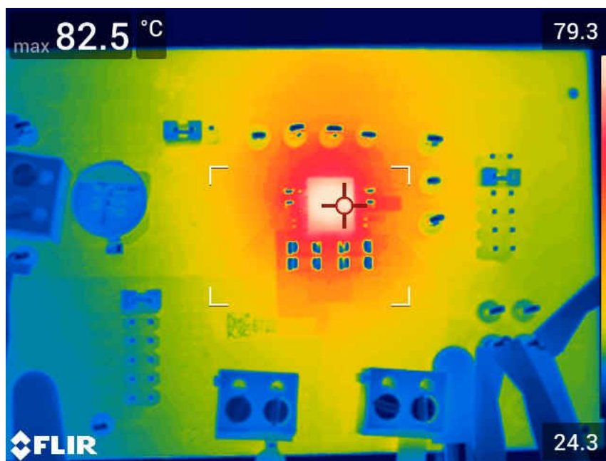
图 10-3. Thermal Image at 25°C Ambient, 12 Vin, 1 Vout, 15 A, 600 kHz
