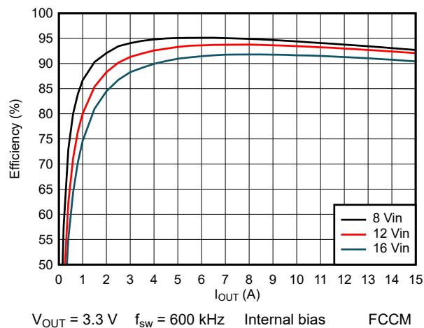
图 8-8. Efficiency
