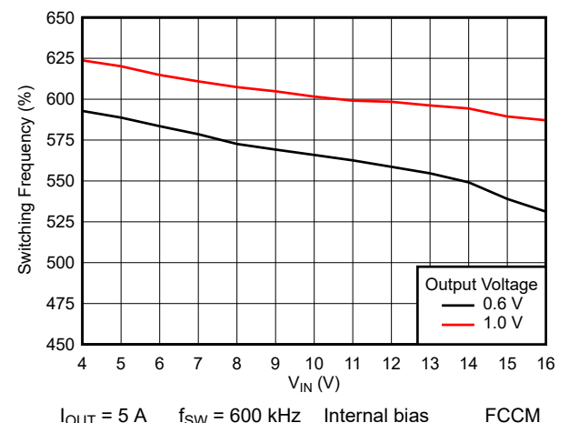
图 8-21. Switching Frequency
