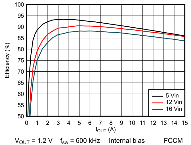
图 8-5. Efficiency
