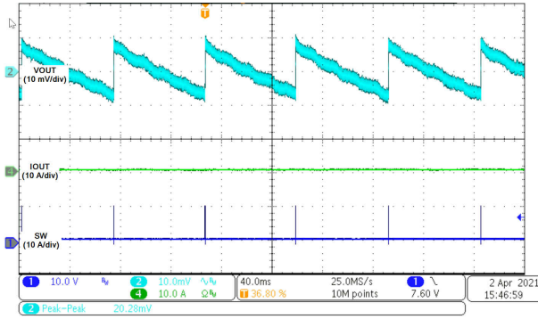
图 8-28. Output Voltage Ripple, V_{RIPPLE} = 20.3\text{ mV}
