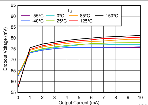
图 5-28. Dropout Voltage vs I_{OUT}
