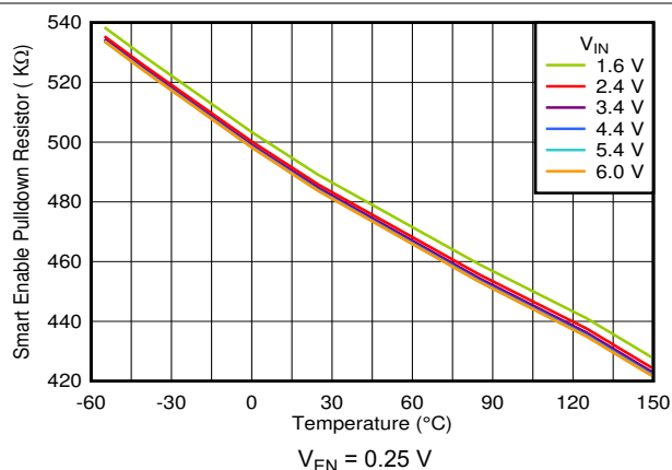
图 5-50. Smart Enable Pulldown Resistor vs Temperature and V_{IN}
