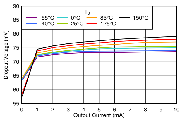
图 5-26. Dropout Voltage vs I_{OUT}
