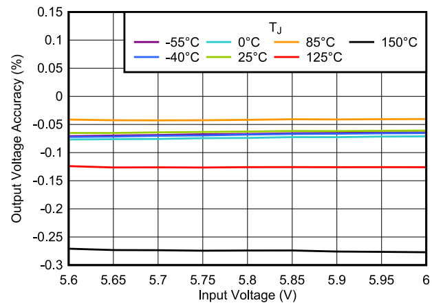
图 5-22. Output Voltage Accuracy vs V_{IN}
