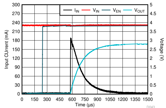
图 5-82. Start-Up
