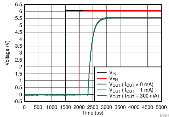
图 5-80. Start-Up
