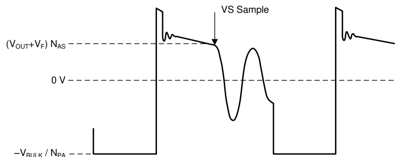
图 7-3. Auxiliary-Winding Voltage
