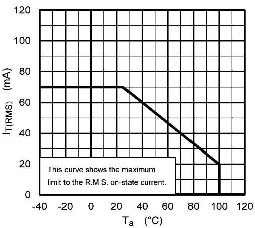
Fig. 12.2 I_T(RMS) - T_a
