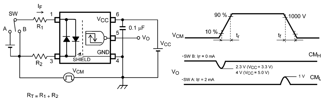
Fig. 12.1.6 Common-Mode Transient Immunity Test Circuit and Waveform
